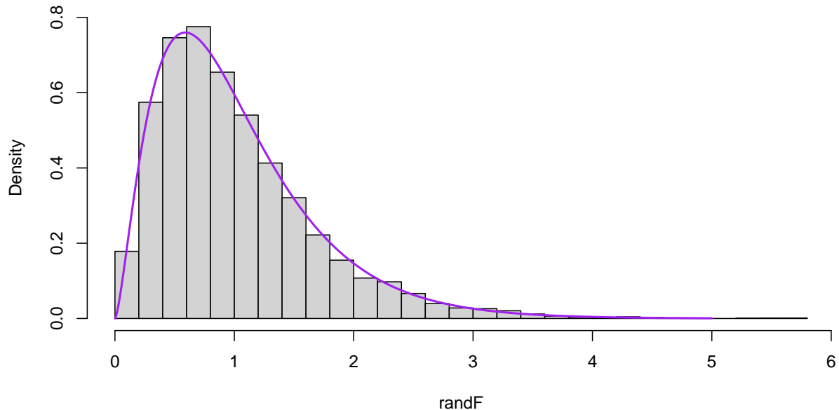
Histogram of randF
